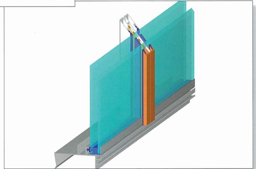
Exclusive range of sections.
